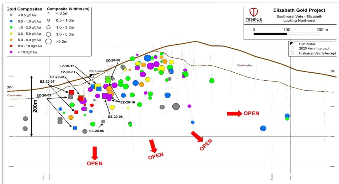
Figure 2- Elizabeth Project Southwest Vein Longitudinal Section
