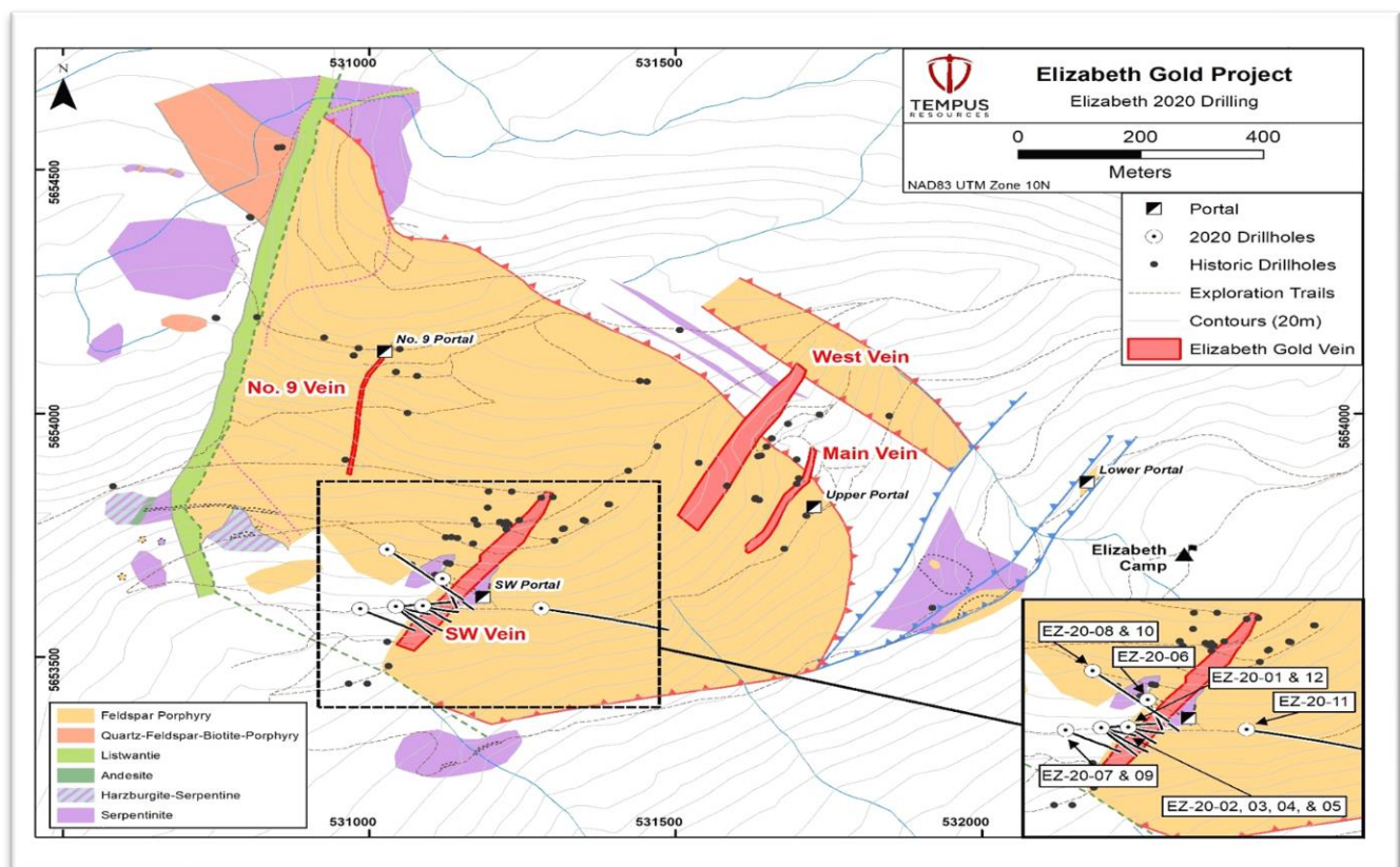
Figure 1- Elizabeth Project Veins and 2020 Drilling
